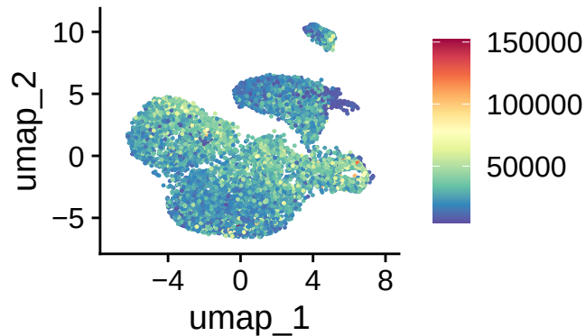
nCount_RNA
