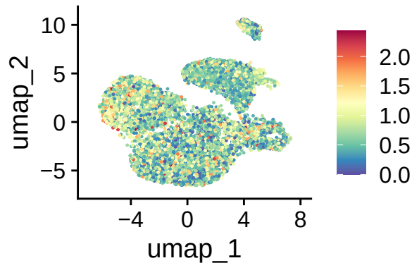
nFeature_RNA
